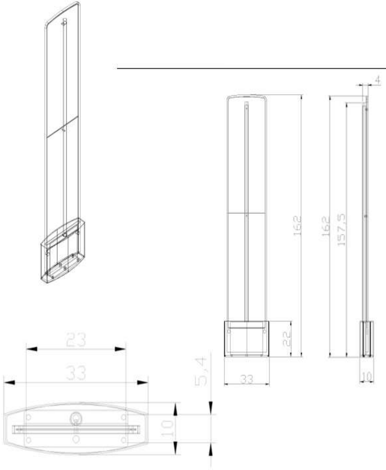
DIMENSION DRAWING
